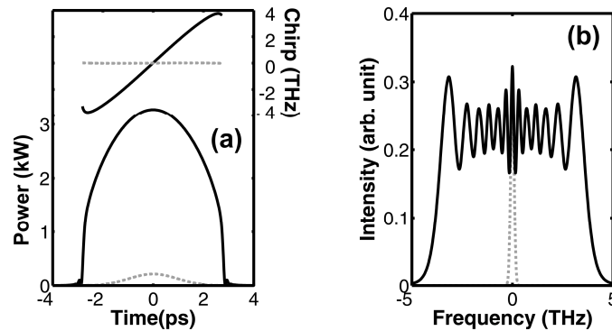
Figure 2. (a) Temporal intensity and chirp profiles, and (b) spectral intensity profiles of the pulse at the entrance (location 1 in Fig. 1; dotted curves) and the exit (location 2 in Fig. 1; solid curves) of the gain fiber.
