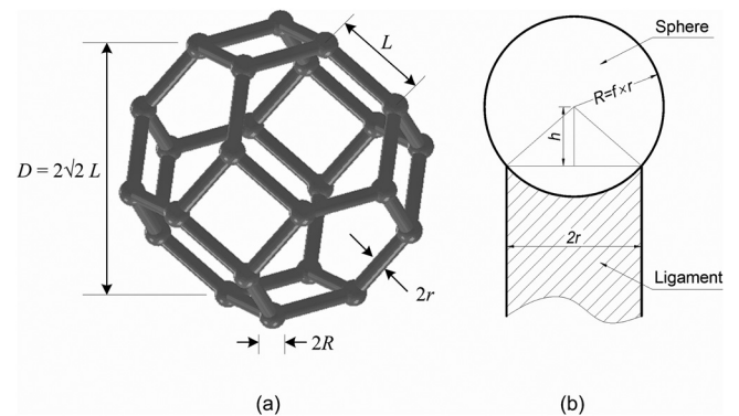
FIG. 3. Basic 3D periodic foam model geometry: (a) a regular truncated octahedron with ligaments of circular cross-section shape (length L , radius r ) and (b) spherical nodes (radius R ) at their intersections. Note that f is a spherical node size parameter, which is set to 1.5.
