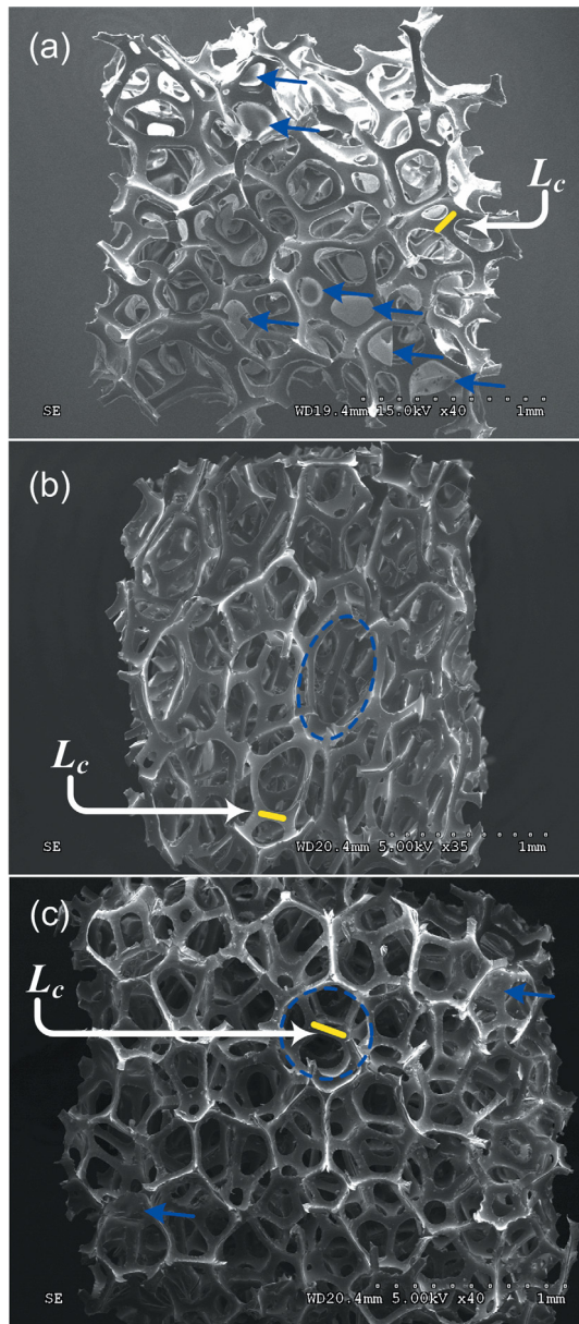
FIG. 8. (Color online) Typical scanning electron microscope images of real foam samples. (a) R_1 , showing a relatively great number of membranes (indicated by arrows) compared to R_2 and R_3 foams. (b) R_2 , having a degree of anisotropy equal to 1.75, as illustrated with a superimposed ellipse. (c) R_3 , exhibits only few isolated residual membranes (thermal reticulation process), with rather spherical pore shapes (schematically represented by a circle). For each real foam sample, a line corresponding to the specific length L_c clearly shows the typical size of an opening which could participate to a critical path.
