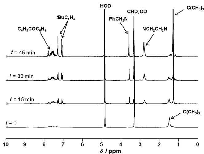
Figure 3. Evolution of the 1 H NMR spectrum of a CD 3 OD solution of 1 (0.5 mL, 5 mM, deoxygenated by freeze pump thaw cycles, sealed tube) upon irradiation of the NMR tube at 365 nm.
