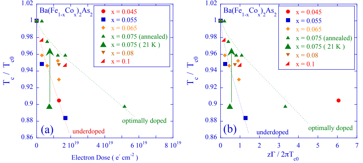
Figure 5. \text{Ba}(\text{Fe}_{1-x}\text{Co}_x)_2\text{As}_2 : evolution of T_c (normalized by the initial critical temperature T_{c0} ) as function of (a) the fluence of 2.5 MeV electrons (b) the estimated normal state scattering rate \Gamma (normalized by T_{c0} ), for different doping levels x . The small data points show the T_c -values after annealing at 300 K. The large green triangle shows the drop of T_c following low-temperature irradiation of optimally doped \text{Ba}(\text{Fe}_{0.925}\text{Co}_{0.075})_2\text{As}_2 , the arrow shows the effect of annealing at 300 K.
