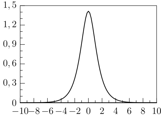
Figure 4. The function \Psi for N = 1 , p = 3 and \omega = 1 .
