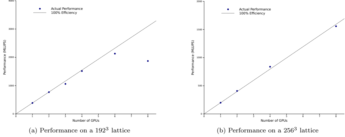
Figure 6: Performance and scalability on a cubic lattice
