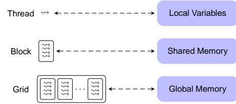
Figure 3: CUDA programming model
