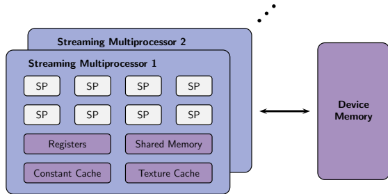
Figure 2: CUDA hardware
