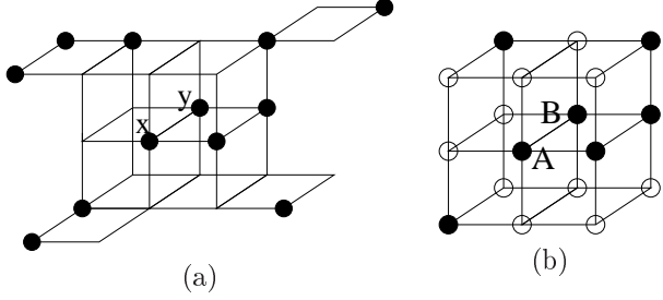
Figure 14: (a): The voxel complex X which is the one of Fig. 10 (a). Here, each voxel of X is represented by a black disk. (b): The mask \mathcal{K}_2 , with A, B matching voxels x, y of X . Condition ii) of Def. 12 for \mathcal{K}_2 is not satisfied but condition i) is fulfilled since the set of voxels \{X_0, \dots, X_7, Y_0, \dots, Y_7\} \cap X is not 0-connected. Thus, by Prop. 13, the voxels x, y constitute a 2-clique of S which is critical for X . See also Fig. 10 (b) where the critical face z = x \cap y is highlighted, we have z_X^+ = \{x, y\} .
