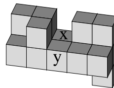
Figure 3: All voxels are simple, the voxels x and y are both “up” voxels.
