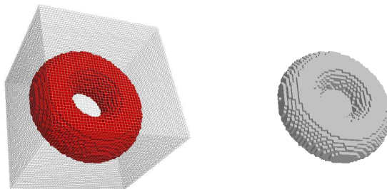
Figure 18: Left: in transparent gray, an object X which is a solid cube; in red, a subset K of X which is a solid torus. Right: the \mathcal{D} -skeleton of X constrained by K . Notice that the hole of the torus has been closed.
