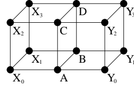
\mathcal{K}_1
