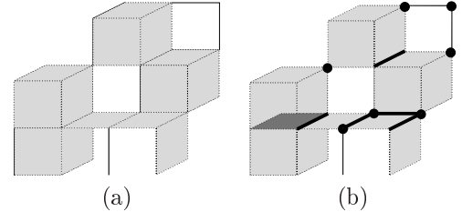
Figure 7: (a) A xel complex X which is made of 3 segments, 3 squares, and 4 cubes, (b) the faces which are essential for X and which are not faces of X are highlighted in dark.
