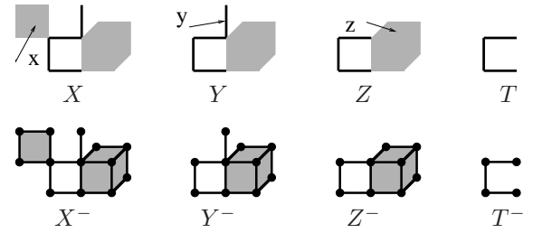
Figure 6: Four xel complexes X, Y = X \setminus \{x\}, Z = Y \setminus \{y\}, T = Z \setminus \{z\} ( X is the xel complex of Fig. 4 (d)). The cubical complexes X^-, Y^-, Z^-, T^- are also given. The face x is simple for X , y is simple for Y , but z is not simple for Z , for Z^- does not collapse on T^- .
