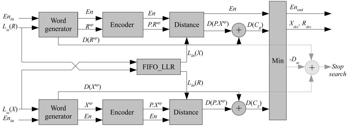
Fig. 2. Code Cortex decoder architecture
