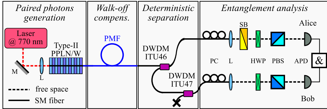
Figure 1. Setup for generating polarization entangled photons at 1540nm using a type-II PPLN/W pumped by a 770nm laser. A PMF is used as birefringence compensator and a set of two DWDMs separates the photons deterministically into the ITU-46/47 channels. A standard Bell inequality apparatus measures the entanglement quality. On Alice’s side, a Soleil-Babinet phase compensator (SB) permits adjusting the phase of the entangled state. L: lens; PC: fiber polarization controller; HWP: half wave-plate; PBS: polarising beam-splitter; &: AND-gate.
