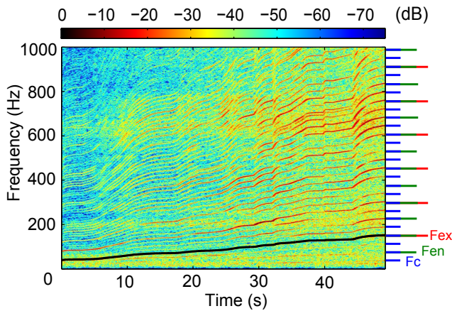
FIG. 3. Spectrogram of a four-cylinder engine noise signal. The solid line is the estimated value of k_{Amax}F_0 (explosion frequency) obtained with the simplified YAAPT method. The signal is sampled at F_s = 44.1 kHz and its spectrogram is calculated using frames of 200 ms zeropadded to 32,768 samples for FFT computations. Hann windows overlapping by 50 % were used. Note that for clarity reasons the spectrogram is showed only for frequencies below 1,000 Hz. On the right of the spectrogram, the colored segments indicate the positions of the harmonics for the last signal frame, as introduced in Figure 1: (red) harmonics of F_{ex} , (green) harmonics of F_{en} and (blue) harmonics of F_c .
