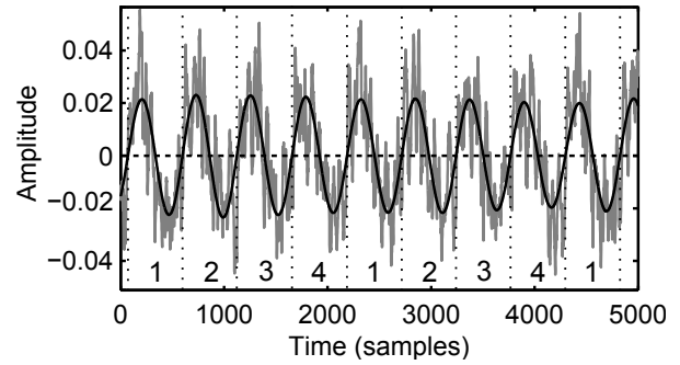
FIG. 4. Segment of a four-cylinder engine noise sampled at 44.1 kHz (gray). Extracted prevailing harmonic of frequency 4F_0 (black). The numbers 1 to 4 indicate the cylinder in which an explosion occurs during the time interval delimited by the dotted vertical lines. Note that the first number is randomly attributed and not associated with a specific cylinder in the engine.
