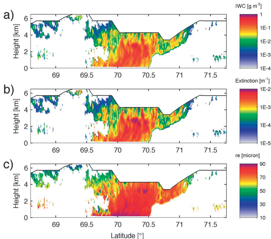
FIG. 3. Latitude–height representation of the synergistic radar–lidar retrieval of ice cloud properties, (a) IWC, (b) visible extinction, and (c) effective radius ( R_e ), for 1 Apr 2008 during the POLARCAT spring campaign.
