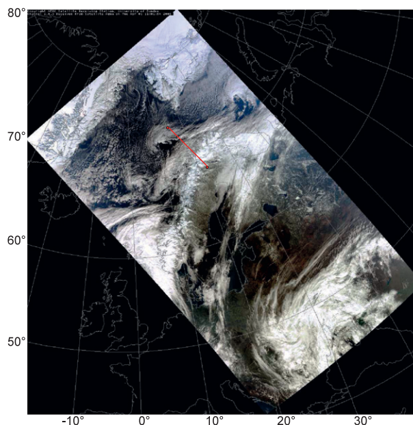
FIG. 1. MODIS visible image above Sweden at 1100 UTC 1 Apr 2008. The flight track corresponding to the study is represented in red.
