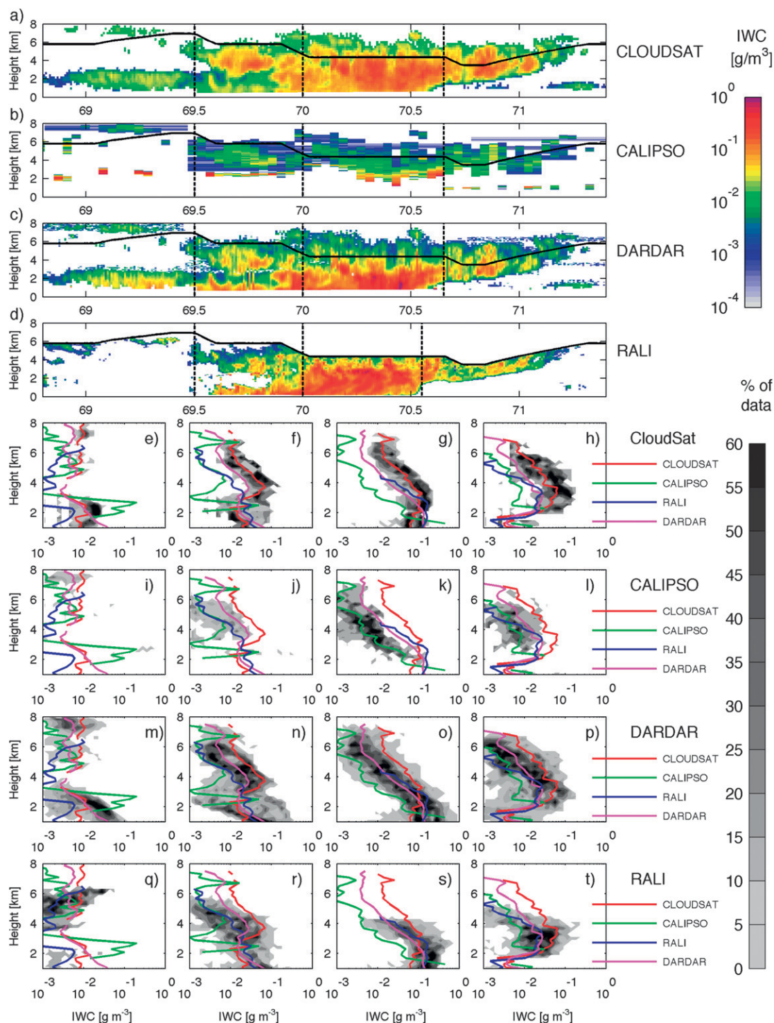
FIG. 9. Comparison between IWC retrieved from RALI, CloudSat , CALIPSO , and DARDAR products for 1 Apr 2008 during the POLARCAT spring campaign. (a)–(d) The latitude height IWC results from CloudSat , CALIPSO , DARDAR, and RALI, respectively. Aircraft altitude is visualized by the black thick line. The scene has been split into the same four different regions as in Fig. 7. For each region, the density distribution plots of IWC vs height are shown for (e)–(h) CloudSat , (i)–(l) CALIPSO , (m)–(p) DARDAR, and (q)–(t) RALI. Pink lines represent the averaged values of DARDAR \log_{10}(\text{IWC}) for each altitude bin, and blue lines correspond to the RALI values. Red and green lines show the averaged values of IWC for the official product from both CloudSat and CALIPSO , respectively.
