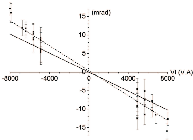
FIG. 3: He-McKellar-Wilkens phase shift as a function of the voltage-current product: the phase \varphi_{final}(V, I) is plotted as a function of the VI product. The data points (squares), represented with their statistical error bars, are in good agreement with a linear behavior \varphi_{final}(V, I) \propto VI , as shown by the best fit to the data (dotted line). The fit slope (-1.68 \pm 0.07)10^{-6} rad/V.A is 31% larger than the expected slope of the HMW phase (full line).
