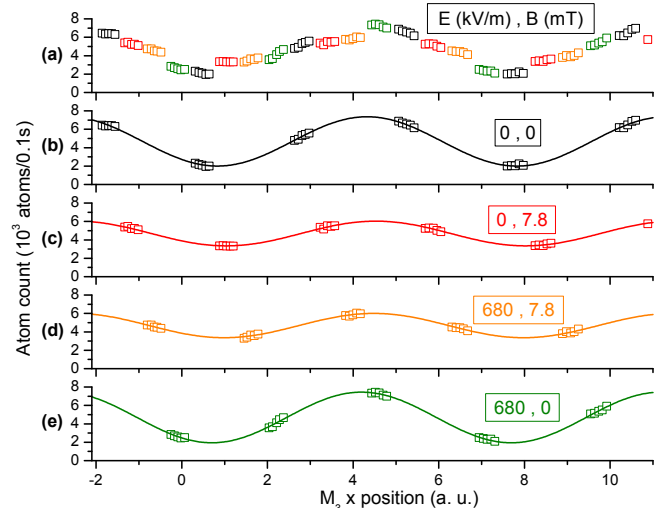
FIG. 2: (Color online) Panel a: the atom interferometer signal is plotted as a function of M_3 x -position, using the 4-field configuration procedure with E = 680 \text{ kV/m} and B = 7.8 \text{ mT} . In panels b-e, the signals corresponding to each field configuration, are plotted with their best fits. The mean detected flux I_0 \approx 47 \times 10^3 \text{ atoms/s} is constant. We use the no-field case as reference for visibility ( \mathcal{V}_0 = (57.2 \pm 0.6)\% ) and phase. In panel c, \mathcal{V}(0, I)/\mathcal{V}_0 = (50.0 \pm 1.2)\% and \varphi_B(I) = -183 \pm 25 \text{ mrad} . In panel d, \mathcal{V}(V, I)/\mathcal{V}_0 = (48.7 \pm 0.2)\% and \varphi_{E+B}(V, I) = -139 \pm 24 \text{ mrad} . In panel e, \mathcal{V}(V, 0)/\mathcal{V}_0 = (102.4 \pm 1.6)\% and \varphi_E(V) = 118 \pm 18 \text{ mrad} . From these measurements, we get \varphi_{EB}(V, I) = (-74 \pm 35) \text{ mrad} . The average over about 100 similar scans produce phase measurements with a few mrad error bar.
