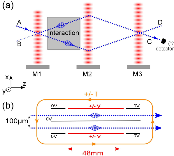
FIG. 1: (Color online) Schematic top views of the setup. Panel a: our atom interferometer, with two entrances A and B and two exits C and D (C is detected). An atomic beam (dotted blue lines) entering by A is diffracted by three quasi-resonant laser standing waves produced by the mirrors M_i . The interaction region is placed where the distance between interferometer arms is largest, close to 100 \mu\text{m} . Panel b: the interaction region producing the electric and magnetic fields (not to scale). The interferometer arms (dotted blue lines) are separated by a septum, which is the common electrode of two plane capacitors producing opposite electric fields (high voltage electrodes in red; grounded electrodes in black). Two rectangular coils (brown rectangle) produce the magnetic field.
