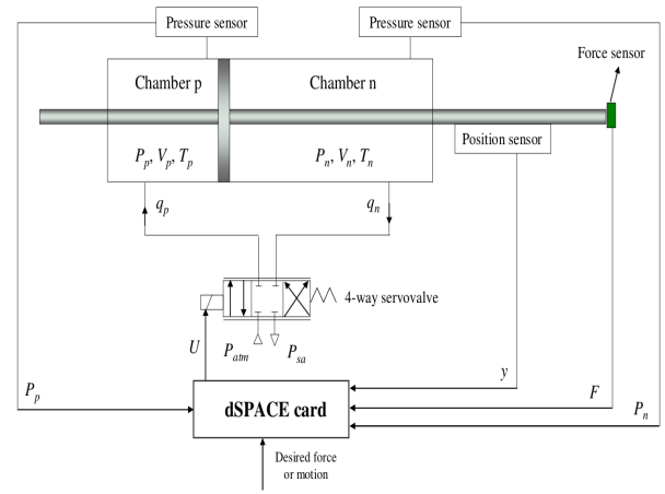
Fig. 1. ELECTRO-PNEUMATIC SYSTEM
