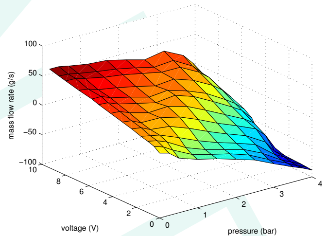
Fig. 2. GLOBAL ATCHLEY SERVOVALVE STATIC CHARACTERISTICS
