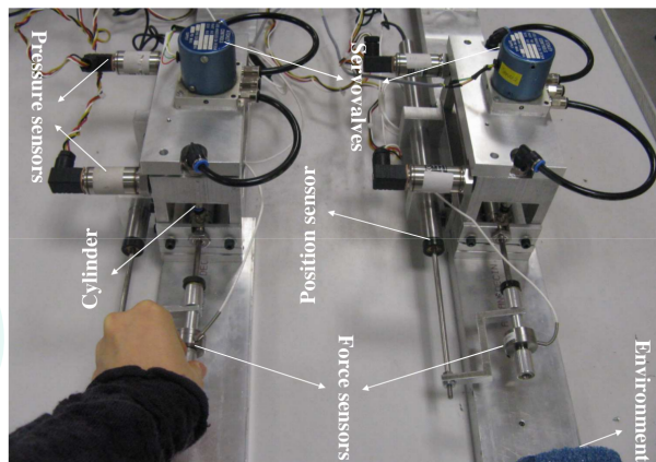
Fig. 12. TELEOPERATION EXPERIMENTAL SETUP USING ELECTRO-PNEUMATIC SERVOVALVES
