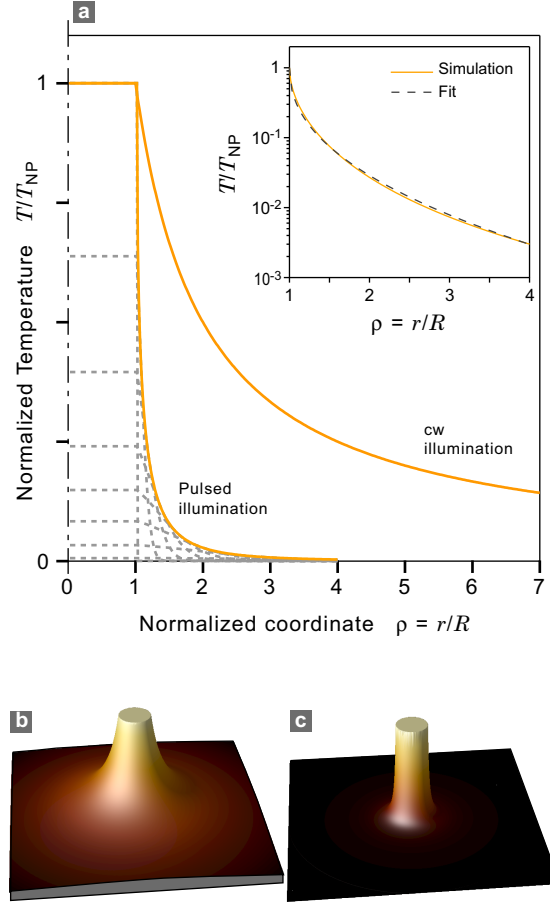
FIG. 4. a) Comparison between the steady state temperature profile under cw illumination and the envelope of the temperature evolution under pulsed illumination. The inset shows the fit of the NP temperature profile in the case of a pulsed illumination. b) Temperature profile around the NP under cw illumination. c) Envelope of the temperature profile over time around the NP during subsequent to a fs-pulse illumination.
