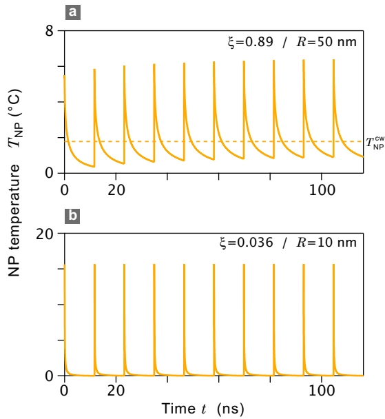
FIG. 8. NP temperature during a series of 10 pulses, f = 86 MHz, \langle I \rangle = 1 mW/ \mu\text{m}^2 , for a NP radius R = 50 nm (a) and R = 10 nm (b). In figure a, the NP temperature corresponding to a cw illumination is T_{\text{NP}}^{\text{cw}} = 1.78^\circ\text{C} and is represented by a dashed line. In the second case, the NP temperature under cw illumination is T_{\text{NP}}^{\text{cw}} = 0.30^\circ\text{C} (not represented).
