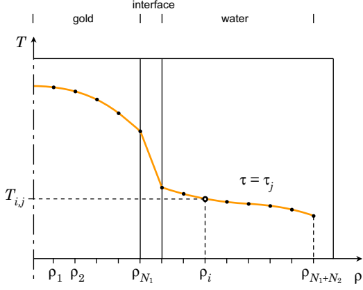
FIG. 10. Schematic of the temperature profile at time \tau_j around a spherical gold nanoparticle as modeled in the FDM-RK4 algorithm. In this second model, the temperature inside the NP is also meshed.
