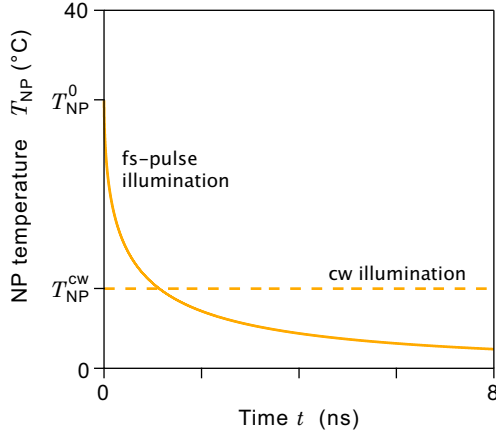
FIG. 2. Evolution of the temperature of a NP a radius R = 50 nm under cw illumination (dashed line) and after a single-pulse illumination (solid line) for a given irradiance \langle I \rangle = 0.1 mW/ \mu\text{m}^2 . This figure aims at defining visually the initial temperature increase T_{\text{NP}}^0 under pulsed illumination and the steady state temperature T_{\text{NP}}^{\text{cw}} under cw illumination. For this particular case, T_{\text{NP}}^0 = 31^\circ\text{C} while T_{\text{NP}}^{\text{cw}} = 9.2^\circ\text{C} .
