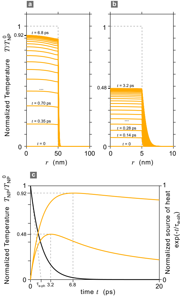
FIG. 6. Temperature rise subsequent to a femtosecond-pulsed illumination for a NP 100 nm in diameter (a) and 10 nm in diameter (b) (interface resistivity 1/g = 0 ). The ideal temperature profile that the NP would achieve if there were no heat release in the surrounding is represented by a dashed line. c) Evolution of the temperature T(r = 0, t) for the two above-mentioned cases along with the normalized heat power p_0(t) (dark line) delivered by the excited electronic gas to the phonons. The normalized temperature does not reach 1 due to heat release during the NP heating.
