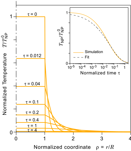
FIG. 3. Result of a numerical simulation showing the universal evolution of the temperature profile for a NP of radius R at different normalized time \tau = a_w t / R^2 . No interface resistivity is considered ( 1/g = 0 ). The inset shows the evolution of the NP inner temperature as function of time.
