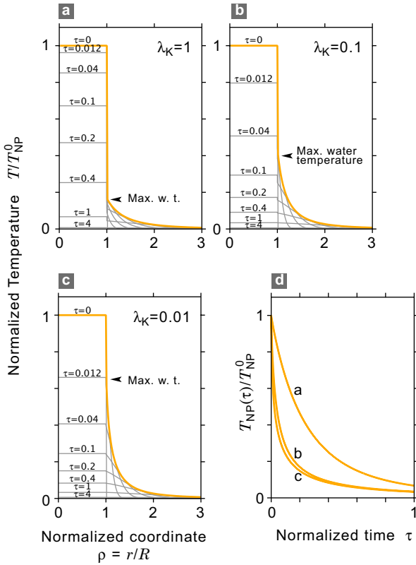
FIG. 5. a, b, c) Temperature envelope of the temperature evolution for three different values of normalized Kapitza length \lambda_K . Temperature profiles are also represented at different times (in gray). d) Evolution of the NP inner temperature corresponding to the three previous situations.
