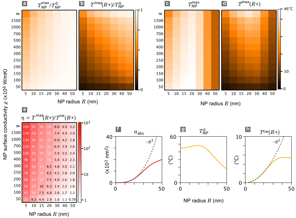
FIG. 7. a) Numerical calculations of the temperature maximum of the NP normalized by the ideal temperature increase T_{NP}^0 for a set of different NP radii and surface conductivities. b) Numerical calculations of the temperature maximum achieved in the surrounding medium normalized by the ideal temperature increase T_{NP}^0 . c) NP maximum temperature when illuminated by a pulsed laser, at a pulsation rate f = 86 MHz and an irradiance I = 0.1 mW/ \mu\text{m}^2 . d) Maximum temperature of the surrounding medium under the same illumination conditions. e) Ratio between the maximum temperature on the NP surface achieved under pulsed illumination and the temperature on the NP surface under cw illumination (Eq. (17)). f) Absorption cross section of a spherical gold NP as function of radius obtained from Mie theory (Eq. (25)) (solid line). The deviation from the R^3 law is represented by a dashed line. g) Ideal temperature increase T_{NP}^0 as function of NP radius. h) Temperature on the NP surface under cw illumination (calculated from Eq. (17)). The deviation from the R^2 law (see Eq. (24)) is represented by a dashed line.
