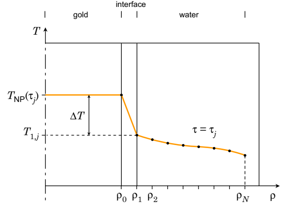
FIG. 9. Schematic of the temperature profile at time \tau_j around a spherical gold nanoparticle as modeled in the FDM-RK4 algorithm. In this first model, the NP temperature T_{NP}(\tau_j) is assumed to be uniform and a temperature discontinuity \Delta T occurs at the nanoparticle interface to take into account a finite interface conductivity.
