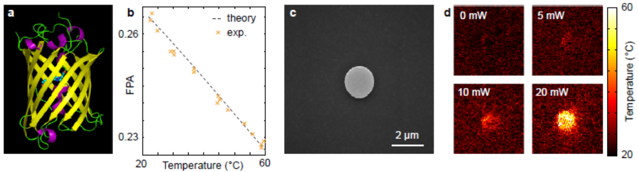
FIGURE. 1. Measuring temperature around micro structures using GFP. a) 3D representation of the structure of GFP. b) Calibration curve that relates between FPA of GFP and temperature in PBS. c) Scanning electron microscope image of a lithographically imprinted gold micro-disc. d) Temperature map obtained around the micro-disc while heating using an infrared laser.
