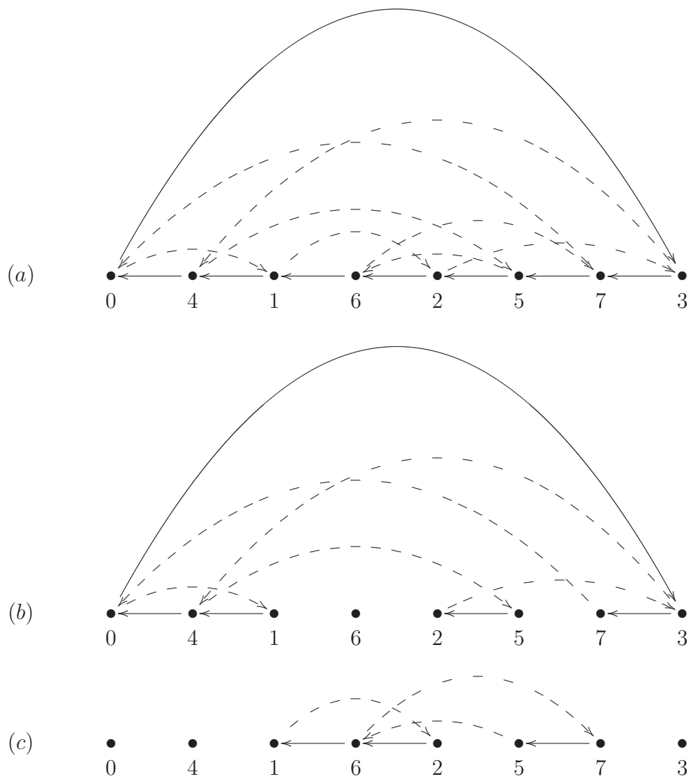
Figure 1: (a) The cycle graph of \langle 4\ 1\ 6\ 2\ 5\ 7\ 3 \rangle ; (b), (c) its decomposition into two alternating cycles
