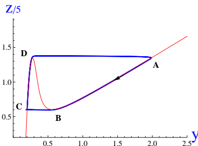
FIG. 9: (Color online) The SM trajectory given by equation (32) for a = 0.65 , b = 4.10^{-3} is the S-shape red curve z(y)/5 , the blue curve is the parametric plot of the 3D flow, i.e. the numerical solution z(x(y(t)), y(t))/5 of equations (26)-(28) for c = b/100 and same values of parameters a, b .
