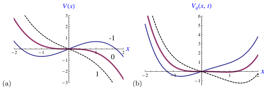
FIG. 5: (Color online) (a) Cubic and (b) quartic potential. The parameter values b = -1, 0, 1 (marked next to the curves) correspond respectively to the blue, thick-red and dashed-black curves.
