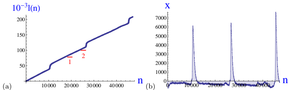
FIG. 2: (Color online) (a) Raw signal 10^{-3}\ell(n) of the wire elongation versus time, in digitalized sensor units. The true elongation is \ell = \ell_n\delta\ell , and the true time is t = n\delta t . (b) Filtered signal x(n) = x_n at the exit of the single pole high-pass filter defined by equation (1).
