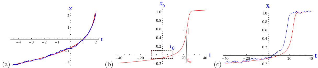
FIG. 6: (Color online) (a) solutions of equation (9), without noise \epsilon = 0 (smooth red curve), and with large amplitude noise ( \epsilon = 1 blue noisy curve). (b) Solution of equation (14) for a = 10^{-3} . The dashed rectangle around the origin defines the region -t_0 < t < t_0 and -1/t_0 < x < 1/t_0 , with t_0 \sim a^{-1/3} . The critical time is t_c(a) \sim 2.34 t_0 . The two small vertical segments delimitate the large slope time duration, of order unity. (c) Solution of equation (19) without noise (smooth red curve) and with large amplitude noise \epsilon = 0.1 , or \tilde{\epsilon}(a) = 1 (blue noisy curve). The two noisy curves in figures (a) and (c) correspond to a single run, with a unique realization of the Langevin equation.
