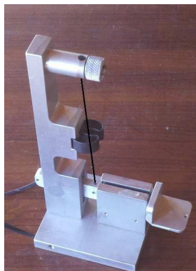
FIG. 1: (Color online) Extensometer used in the experiment.
