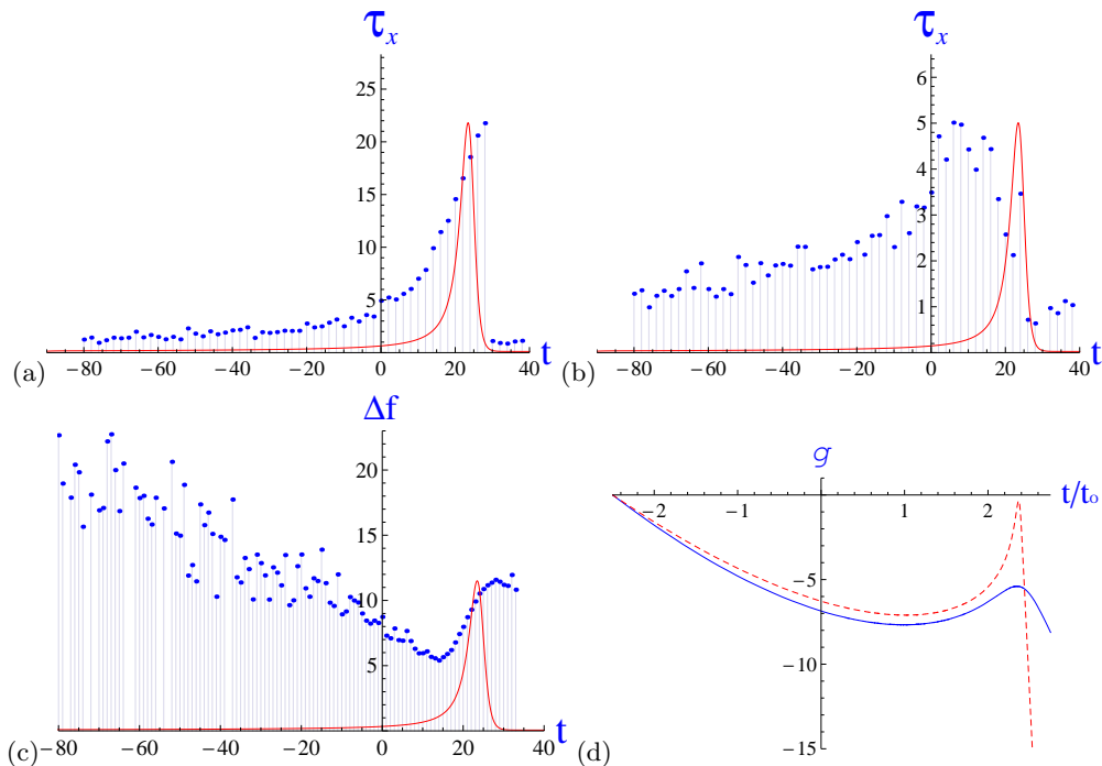
FIG. 7: (Color online) (a-b) Correlation time \tau_x of the fluctuation x(t) - x_0(t) for the saddle-node model (19) with a = 10^{-3} . The correlation functions are defined by equation (22) and (23) for curves (a) and (b) respectively; (c) Spectral width (a. u.) calculated with w_g = t_0 , for a = 10^{-3} ; the red curves display the time derivative x(t) in order to indicate the catastrophe time. (d) g(t/t_0) for a = 10^{-3} (solid, blue), and a = 10^{-6} (dashed, red).
