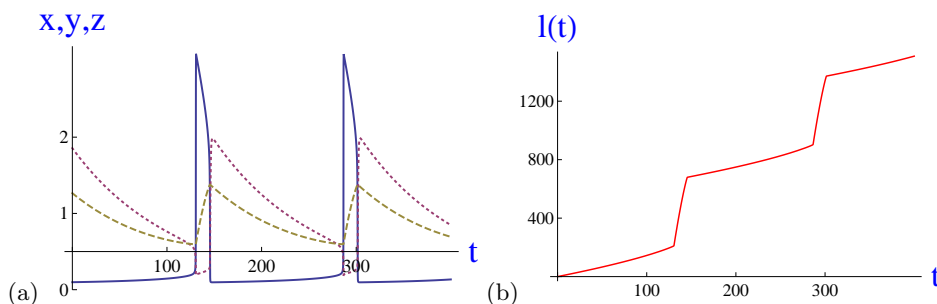
FIG. 8: (Color online) (a) Densities of mobile, immobile, and Cottrell's dislocations as function of time, solution of the 3D flow (26)-(28) for a = 0.65 , b = 410^{-3} , and c = b/100 . The three curves are 0.08x(t) (solid), y(t) (dotted) and z(t)/5 (dashed), (b) Creep signal \ell(t) .
