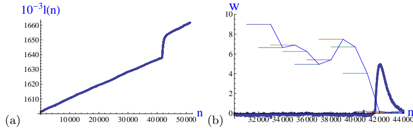
FIG. 4: (Color online) Example of data with a single avalanche. (a) Elongation versus time, \ell(n) , in sensor units. (b) Ten successive values of the width w_i of the cumulative spectra (before the burst) in arbitrary units, taken into the time interval 32000\delta t < t < 42000\delta t ( or 32000 < n < 42000 ). The sequences (n_i, n_i + N) overlap with N = 2000 and n_{i+1} - n_i = 1000 . The horizontal segments indicates the time interval over which the width is calculated. The broken thin line joins the values of w_i taken at the end of each sequence, at time (n_i + N)\delta t to simulate an experimental observation performed in real time. The thick filled curve displays the filtered signal x_n which indicates the avalanche time.
