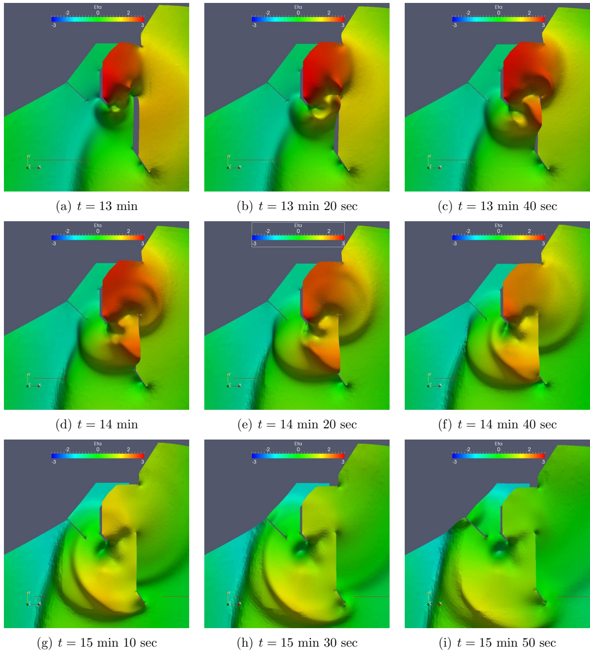
FIGURE 21. Free-surface close up between 13 and 16 minutes.
