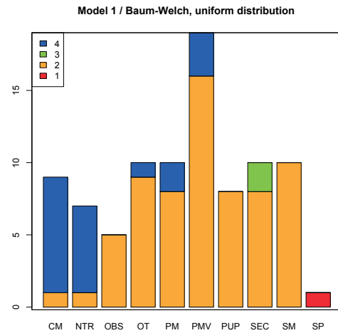
(b) Baum–Welch
