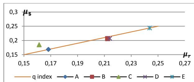
Figure 6: Graphic representation of alternatives in the plane (\mu_r, \mu_s) ( \delta = 0.1, q = 1 ).
