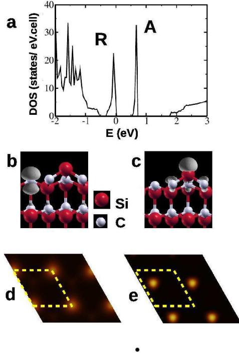
FIG. 2: (color on line) Electronic structure of the (2 \times 2)_C reconstruction of the C-terminated SiC surface. (a) density of states, (b) (resp. (c)) isocontours of |\psi|^2 integrated on the energy range of peak R (resp. A), superimposed to the ball and stick model of the surface. (d) (resp. (e)) section of (b) (resp. (c)) just above the adatom. (d) ( resp. (e)) can be compared to a filled (empty) state STM image
