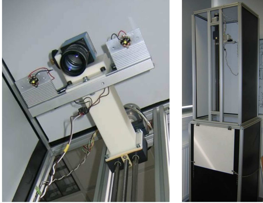
Fig. 2. Acquisition system
