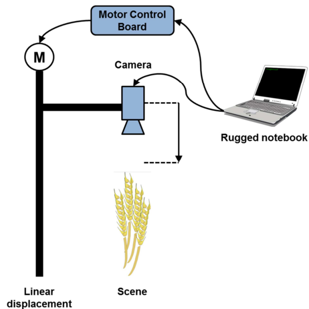
Fig. 1. Acquisition process
