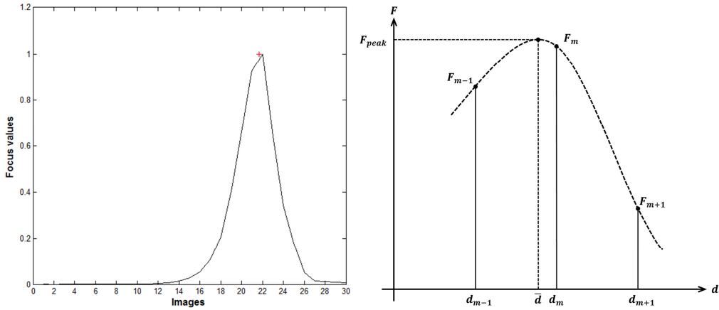
Fig. 3. Focus measure curve and Gaussian approximation
