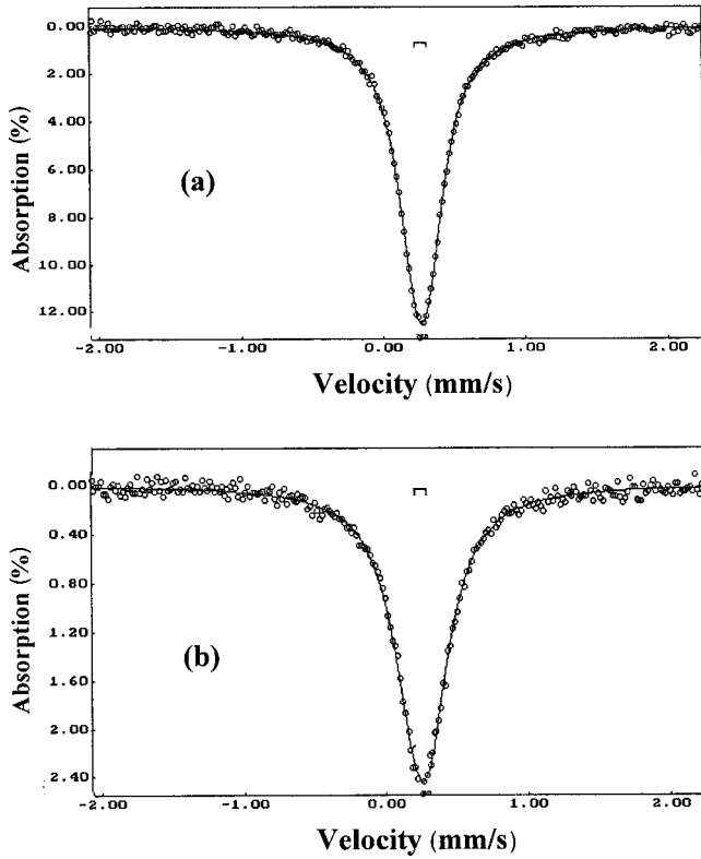
FIG. 2. 57 Fe Mössbauer spectra of (a) NdNi 0.98 Fe 0.02 O 3 and (b) SmNi 0.98 Fe 0.02 O 8 at room temperature.
