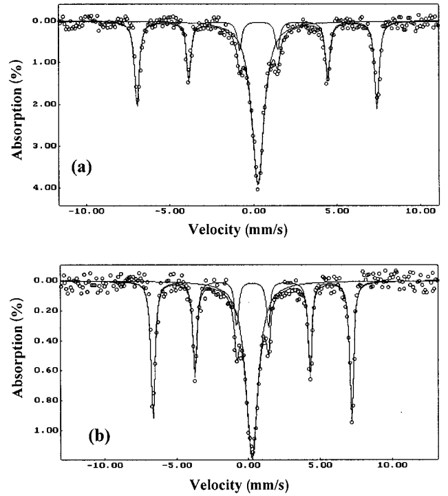
FIG. 3. 57 Fe Mössbauer spectra of (a) NdNi 0.98 Fe 0.02 O 3 at 60 K and (b) SmNi 0.98 Fe 0.02 O 8 at 80 K.
