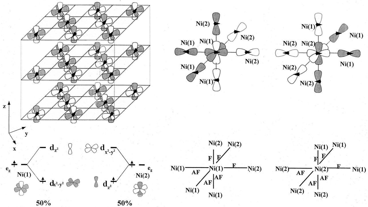
FIG. 1. Magnetic arrangements of the Ni moments in the ANiO_3 ( A = Nd, Sm ) at T < T_N . The different shading of the octahedra corresponds to the occupation of either d_{z^2} - or d_{x^2-y^2} -type orbitals and local magnetic surrounding of Ni(1) and Ni(2) cations.
