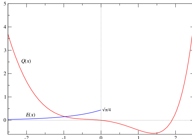
FIG. 1. Plot of Ebeling direct and exchange functions Q(x) and E(x) .
