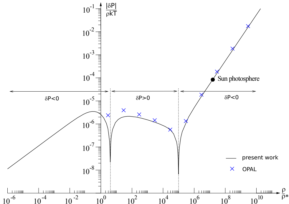
FIG. 4. Logarithmic plot of deviations to Saha pressure for pure hydrogen along isotherm T = 6000 K. ( \rho^* = 2.12 \times 10^{15} \text{ m}^{-3} ). Crosses correspond to tabulated points of the OPAL equation of state [4] (with corrected ground-state energy [36]).
