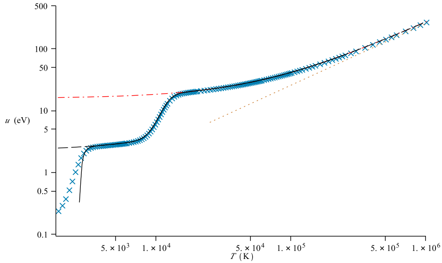
FIG. 8. Internal energy per proton along isochore 10^{-8} g/cc according to SLT EOS (black line), OPAL EOS (crosses) and Saha EOS (dashed line). For the difference between the two former and the latter curves, see Fig. 9. All energies are shifted upwards by |E_{H_2}|/2 . The plot shows also curves |E_{H_2}|/2 + 3kT (red dot-dashed line) and 3kT (dotted line).
