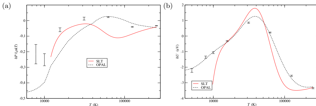
FIG. 11. Deviations (with respect to ideal Saha values) of pressure (a) and internal energy per electron-proton pair (b) as a function of temperature along isochore 0.0125 g/cc, according to SLT EOS (red line) and OPAL EOS (dashed line). Points are simulation results of Ref. [7].
