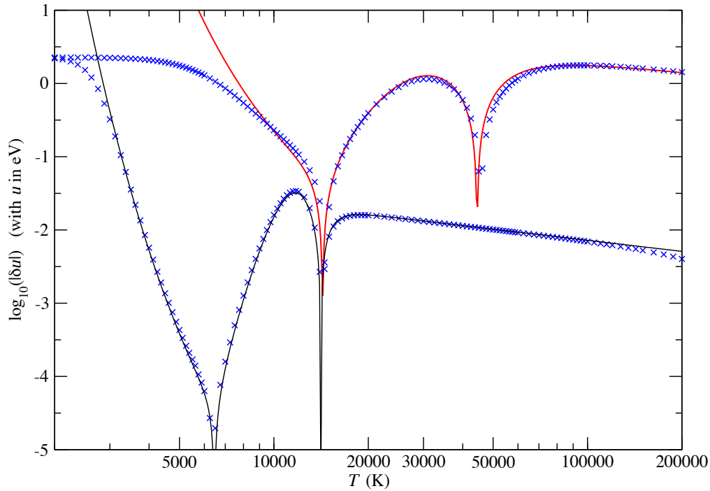
FIG. 9. Deviations to Saha internal energy for isochores 10^{-8} g/cc (black line) and 10^{-3} g/cc (red line) according to the SLT EOS. Crosses denote tabulated points of the (corrected) OPAL EOS.
