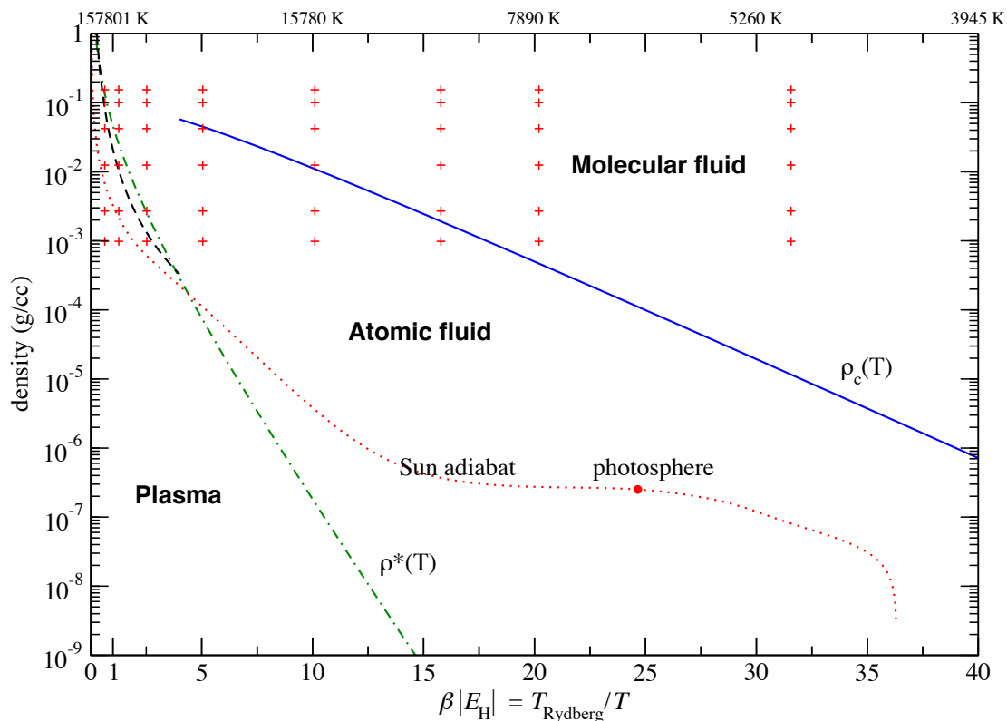
FIG. 12. Phase diagram of a pure hydrogen gas at low densities. The crosses denote state points where simulation results are available [7]. The crossover density \rho^*(T) between the plasma and the atomic phase (dot-dashed line) gives essentially the borderline of the validity domain of the standard virial expansion, which applies only in the plasma phase. The dashed line corresponds to a plasma coupling parameter \Gamma = 0.5 . The SLT expansion is valid in both the plasma and atomic phases, up to the blue line \rho_c(T) [eq. (57)] which locates the cross-over to the molecular phase. The state point of the Sun photosphere, and the track of the Sun adiabat (dotted line) are also shown.
