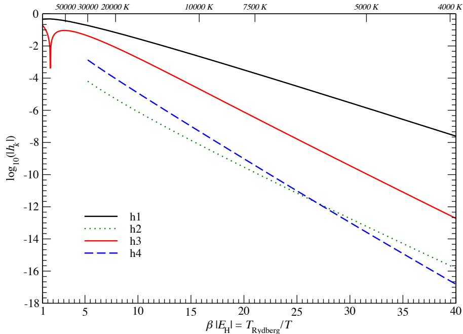
FIG. 3. Plot of functions h_k(\beta) . The scale for \beta is in Rydberg.
