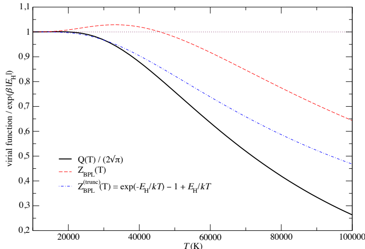
FIG. 2. Comparison of the Brillouin-Planck-Larkin partition function (red dashed curve) to the exact virial function Q(x_{pe}(T)) (black line) for temperatures up to 100 000 K. Truncating the sum in Z_{BPL} after the first term yields a quite good approximation (dot-dashed curve). The dotted line (constant value 1) corresponds to keeping only the groundstate contribution \exp(-E_H/kT) .
