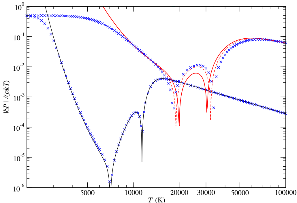
FIG. 7. Deviations to Saha pressure along isochores 10^{-8} g/cc (black line) and 10^{-3} g/cc (red solid line) according to the SLT EOS. Crosses correspond to values of the (corrected) OPAL EOS. The dashed line shows the effect of neglecting term P_4 in the SLT EOS.
