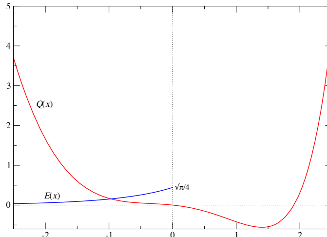
FIG. 1. Plot of Ebeling direct and exchange functions Q(x) and E(x) .
