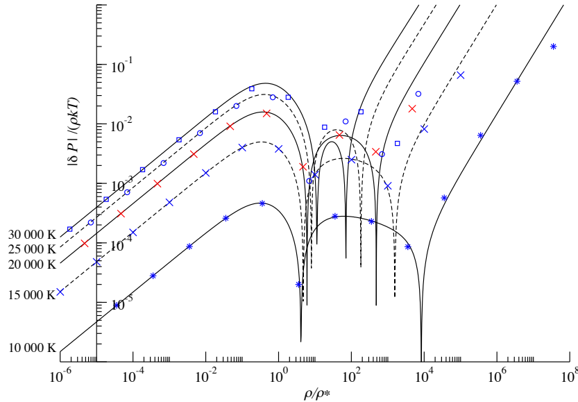
FIG. 5. Logarithmic plots of deviations to Saha pressure along isotherms from 10\,000 K up to 30\,000 K according to the SLT EOS (solid and dashed lines) and to the tabulated OPAL EOS (symbols).
