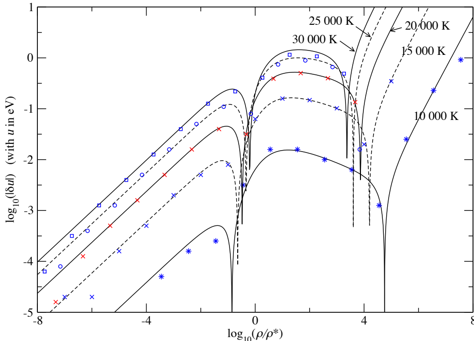
FIG. 6. Deviations to Saha internal energy for isotherms between 10 000 K and 30 000 K according to the SLT EOS. Points of the (corrected) OPAL EOS are shown by symbols (up to density 0.1 g/cc).
