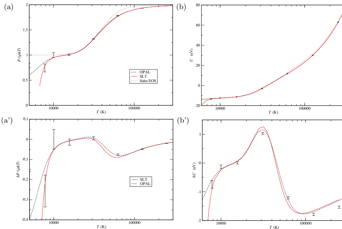
FIG. 10. Pressure (a) and internal energy (b) per electron-proton pair as a function of temperature along isochore 10^{-3} g/cc, according to SLT EOS (red line), OPAL EOS (dashed line), and ideal Saha EOS (dotted line). Points are simulation results of Ref. [7]. Plots (a') and (b') show deviations to the ideal Saha values along the isochore.
