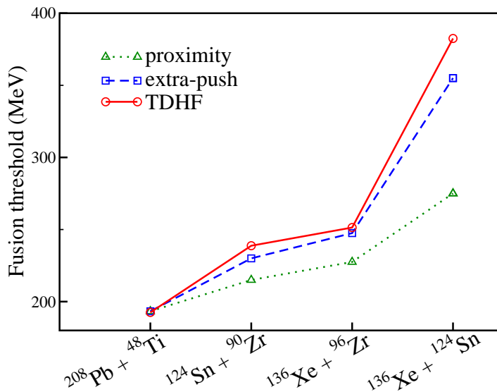
Figure 8. TDHF fusion thresholds for several heavy systems are compared with the proximity barrier [59] and with results from the extra-push model [58].
