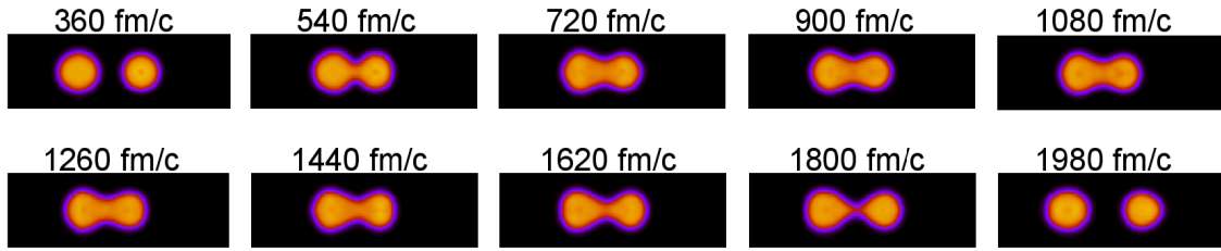
Figure 9. Density profile in the ^{90}\text{Zr}+^{124}\text{Sn} head-on collision at E_{c.m.} = 235 MeV. From Ref. [60].
