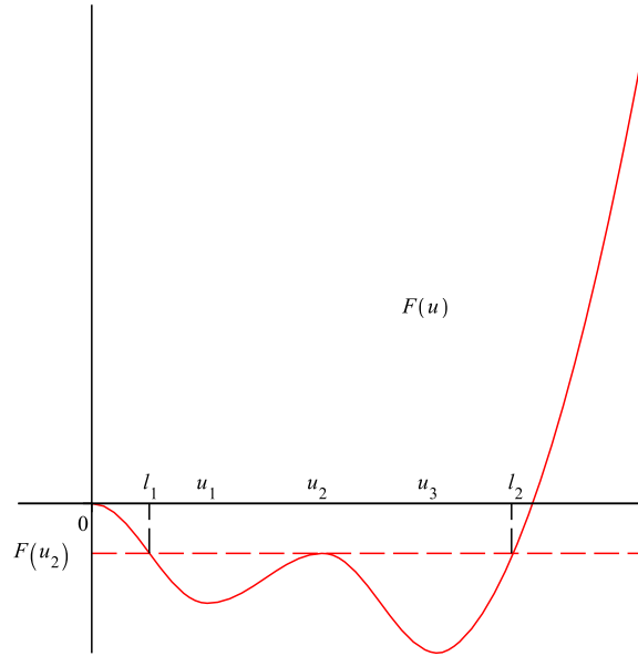
FIGURE 4. If \ell_1 \neq \ell_2 , then 0 < \ell_1 < u_1 and u_3 < \ell_2 < A .
