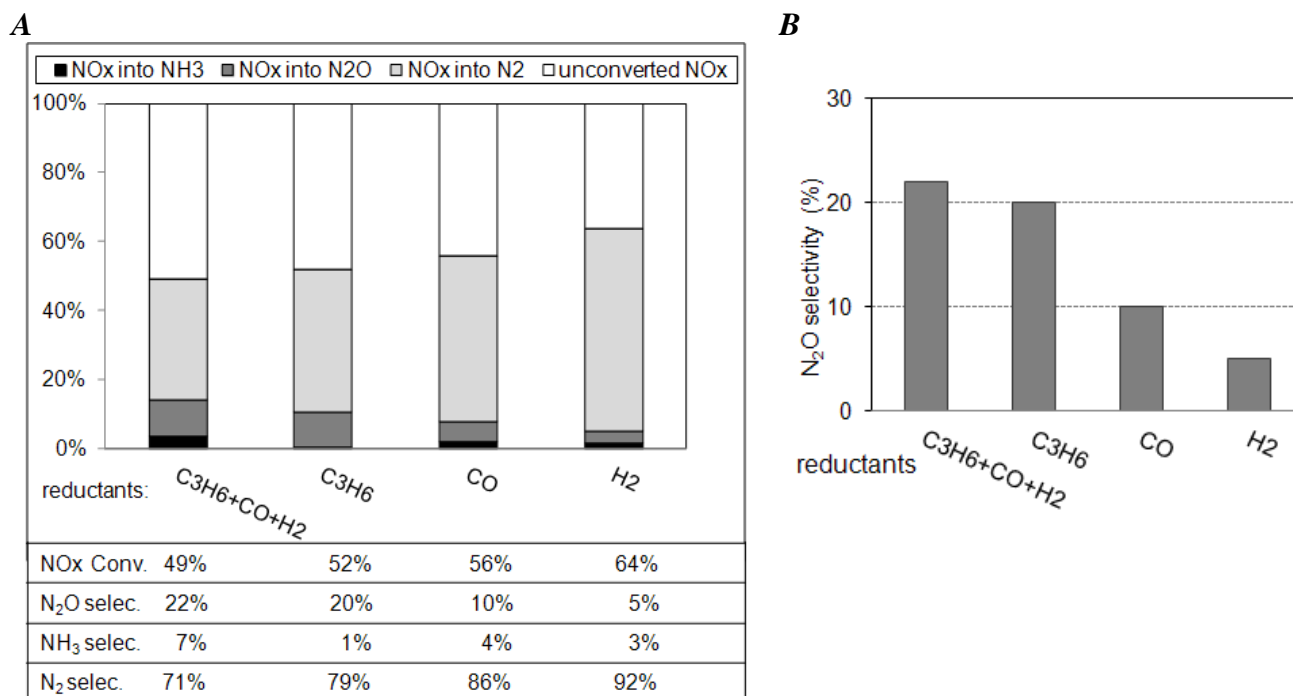
Figure 4: Pt/CZ catalyst (70mg): NO_x removal efficiency (A) and N_2O selectivity (B) obtained at 300^\circ C depending on the introduced reducer(s) (same in both lean and rich gas mixture).
