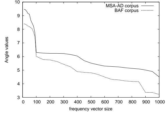
Fig. 2. The cosine similarity for BAF and MSA-AD corpora
