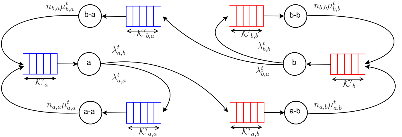
Figure 1: VSS stochastic model: A closed queuing network with periodic time-varying rates.
