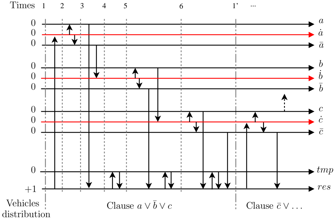
Figure 4: Reduction of 3-SAT to FCFS FLOW STATION CAPACITIES. Example with clauses (a \vee \bar{b} \vee c) \wedge (\bar{c} \vee \dots) .
