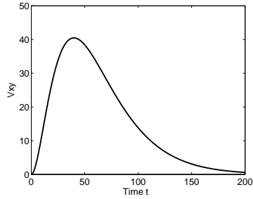
Fig. 7. V_{xy}(t) as a function of time.
