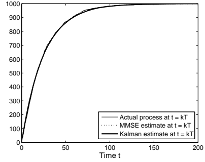
Fig. 10. Performance of MMSE estimation and Kalman filter estimation of the process with Scenario 5.
