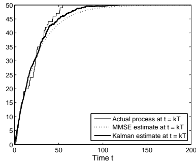
Fig. 3. Performance of MMSE estimation and Kalman filter estimation of the process for Scenario 2.
