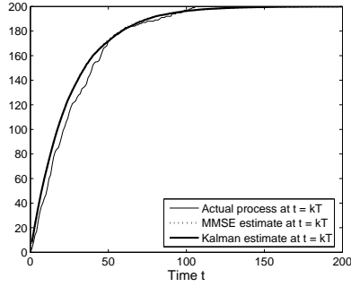
Fig. 9. Performance of MMSE estimation and Kalman filter estimation of the process with Scenario 4.
