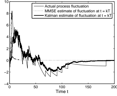
Fig. 6. MMSE estimation and Kalman filter estimation of the process fluctuations for Scenario 3.
