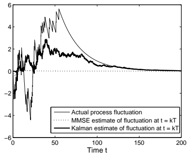
Fig. 4. MMSE estimation and Kalman filter estimation of the process fluctuations for Scenario 2.
