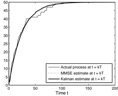
Fig. 1. Performance of MMSE estimation and Kalman filter estimation of the process for Scenario 1.
