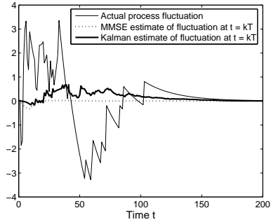
Fig. 2. MMSE estimation and Kalman filter estimation of the process fluctuations for Scenario 1.
