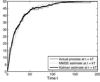
Fig. 5. Performance of MMSE estimation and Kalman filter estimation of the process for Scenario 3.
