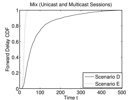
Fig. 12. Comparison of forward delay CDF of scenario D versus scenario E: mix of 50% unicast and 50% multicast sessions.
