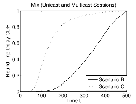
Fig. 6. Comparison of round trip delay CDF of scenario B versus scenario C: mix of 50% unicast and 50% multicast sessions.
