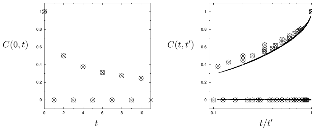
Figure 1. Correlations C(t, t') calculated via numerical solution of (49) (for t, t' \leq 10 , circles) versus correlations measured in numerical simulations with N = 10^6 (crosses). Here T = 0.1 and \tilde{P}(J, \theta) = \frac{1}{2}\delta(\theta)[\eta\delta(J-1) + (1-\eta)\delta(J+1)] (which can be mapped onto the non-disordered Ising chain). Left: values of C(t, 0) , i.e. overlap with the initial state, plotted versus t (which decays as a power law). Right: correlations C(t, t') plotted versus the ratio t/t' , for t, t' = 1 \dots 10 . Dots show the values of C(t, t') for larger times 50 \leq t \leq t' \leq 100 , as measured in simulations, showing the typical nonequilibrium behaviour C(t, t') \sim C(t/t') of the ageing regime. Upper branches: even values of t - t' ; lower branches: odd values of t - t' .
