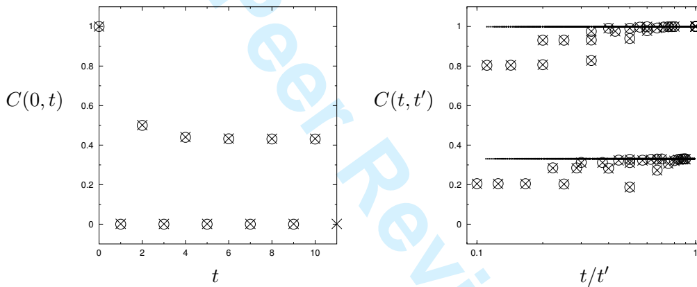
Figure 2. Correlations C(t, t') calculated via numerical solution of (49) ( t, t' \leq 10 , circles) versus correlations measured in numerical simulations with N = 10^6 (crosses). Here T = 0.1 and \tilde{P}(J, \theta) = \frac{1}{4}[\delta(\theta - \frac{1}{2}) + \delta(\theta + \frac{1}{2})][\eta\delta(J-1) + (1-\eta)\delta(J+1)] , i.e. weak random fields. Left: values of C(t, 0) , i.e. overlap with the initial state, plotted versus t . Right: correlations plotted versus the ratio t/t' , for t, t' = 1 \dots 10 . Dots show the values of C(t, t') for larger times 50 \leq t \leq t' \leq 100 , as measured in simulations. Upper branches: even values of t - t' ; lower branches: odd values of t - t' . The system stabilises into a meta-stable state on the timescales considered, from which it takes significantly more time to escape.
