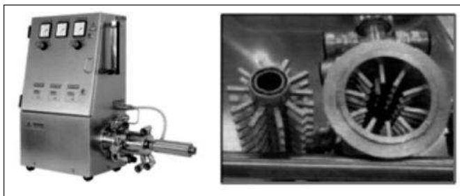
Figure 3: Example of an industrial foam gun (stator and rotor details).
