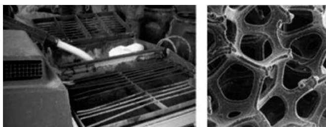
Figure 4: left: Adding foam in the gauging chamber of a mixer. Right: Foam deposit on a metal substrate (www.recemat.nl).
