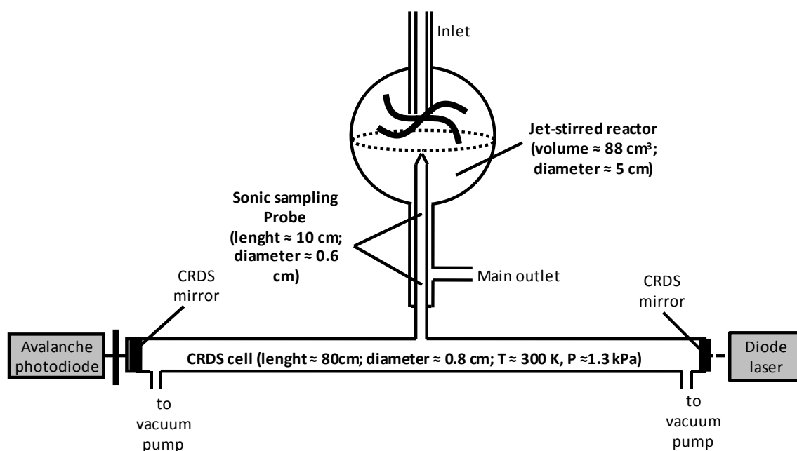
Figure 2. Simplified scheme of the experimental device.
