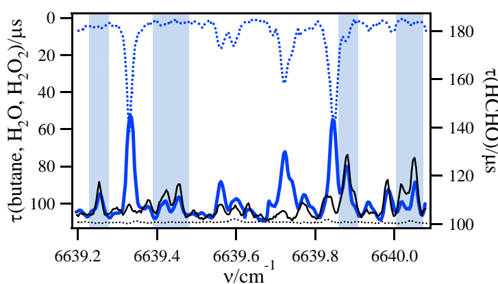
Figure 3. Typical CRDS spectrum obtained for the oxidation of n -butane at 650 K (thick full blue line) compared to the spectrum of \text{H}_2\text{O}_2/\text{H}_2\text{O} mixture (thin full black line), \text{H}_2\text{O} (thin dotted black line), and \text{HCHO} (thin broken blue line, right axis). Shaded areas show \text{H}_2\text{O}_2 absorption lines which are not disturbed by other absorbing species.
