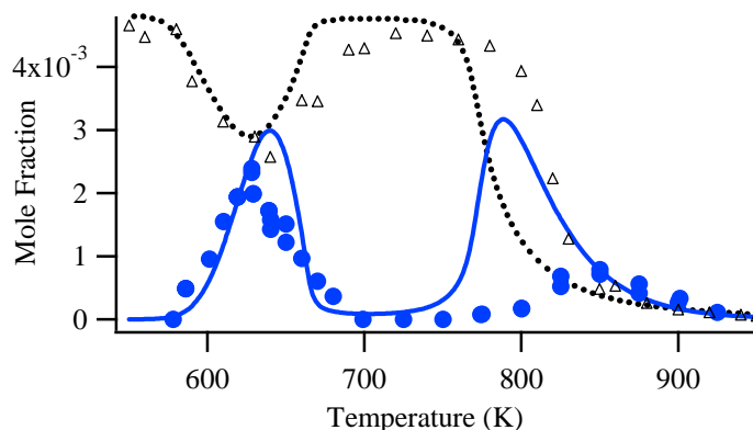
Figure 4. Evolution with temperature of the experimental (points) and computed (lines) mole fractions of n -butane (white triangles and dotted line, mole fraction/5) and hydrogen peroxide (blue dots and full line).
