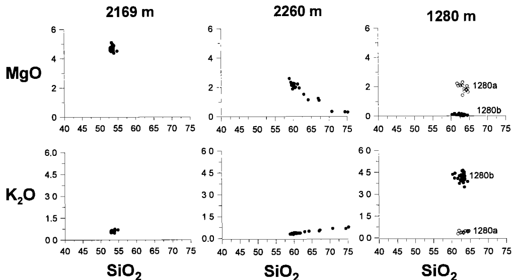
Figure 4. Electron microprobe analysis for layers at 2169 m (20 shards), 2260 m (20 shards), and 1280 m (47 shards) plotted on Harker diagrams of K 2 O versus SiO 2 and MgO versus SiO 2 . The 1280 m layer is divided in two subgroups 1280a and 1280b.
