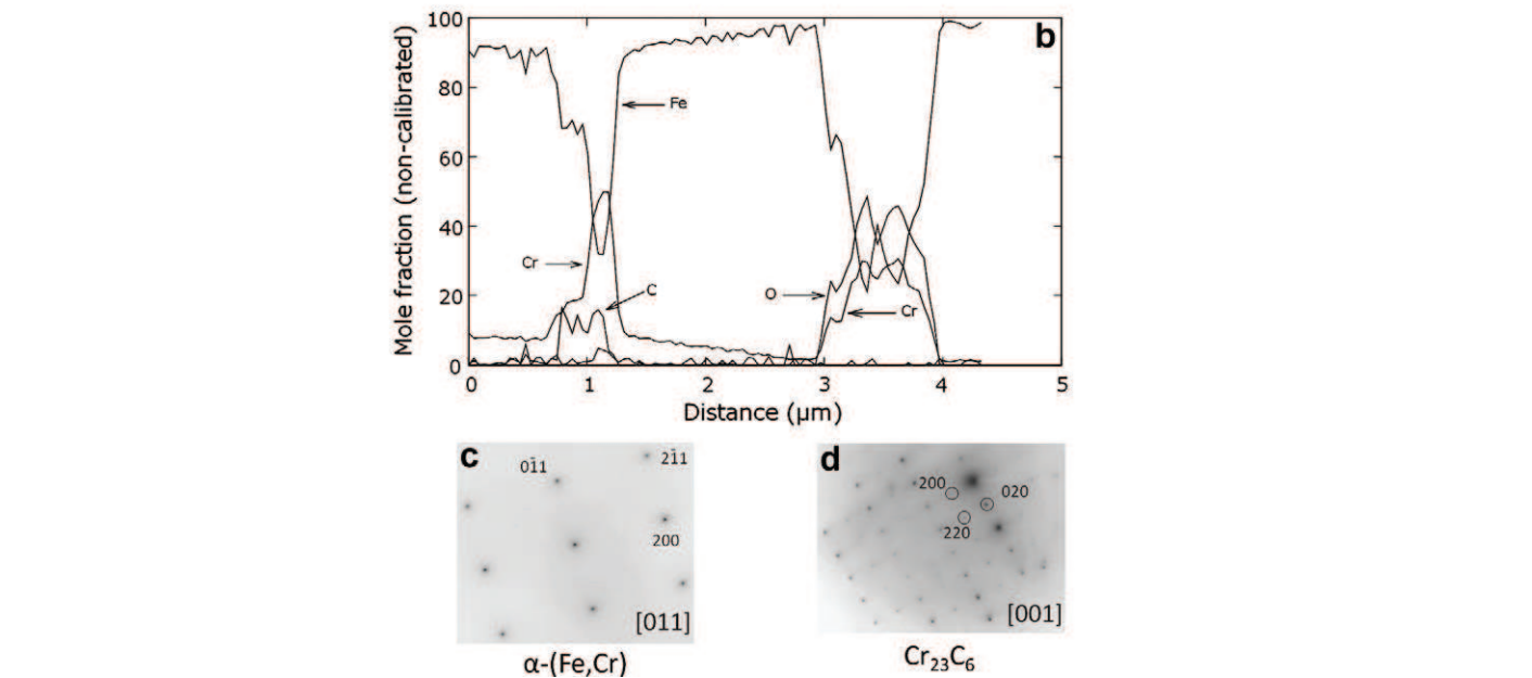
Fig. 12. TEM analyses at the interface between internal oxidation and carburisation areas in Fe-9Cr after 20 h exposure to Ar-20CO 2 at 800 °C. (a) Bright field image and corresponding EDS elemental maps; (b) EDS linescan; (c) and (d) selected area diffraction pattern of the \alpha matrix ([011] zone axis) and of a (Cr,Fe)_{23}C_6 carbide ([001] zone axis), respectively. The arrow and star in (a) indicate the location of the linescan in (b) and of the pattern in (d), respectively.
