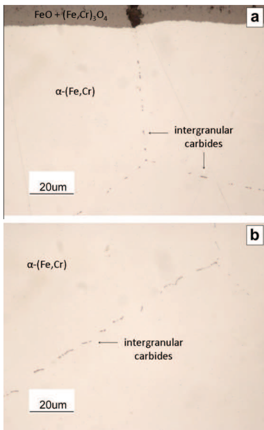
Fig. 4. Intergranular carburation of Fe-2.25Cr after 120 h exposure to Ar-20CO 2 at 650 °C, etched with Murakami's reagent. (a) Scale/alloy interface; (b) deep within the alloy.
