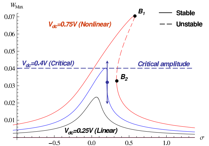
Fig. 3. Forced frequency responses of the typical resonator described in Fig. 1 for h = 0.5 \mu\text{m} and Q = 5000 . \sigma is the detuning parameter and W_{max} is the displacement of the beam normalized by the gap g_d at its middle point \frac{l}{2} . B_1 and B_2 are the two bifurcation points of a typical hardening behavior.
