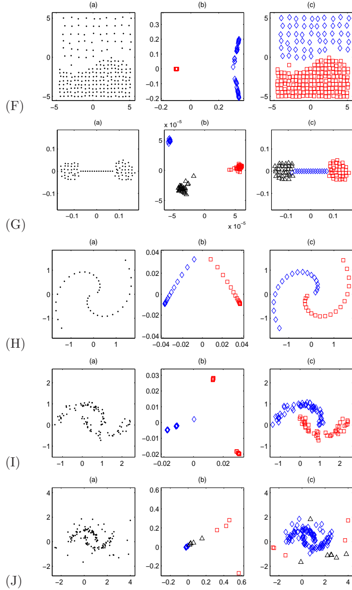
Figure 3: F: Different constant densities; G: 2 clusters and constant density link; H: 2 spirals; I: 2 moons.; J: 2 moons and outliers. Left (a) : Data; Middle : DRPT-MDS embedded data; right : data labelled with clustering labels obtained by k-means method on the DRPT-MDS embedded data. Note that when outliers are present, k-means was set to search 3 clusters.
