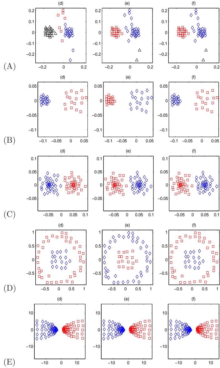
Figure 5: Data sets A to E are those already explored for Figure 2. Left(d) : Spectral clustering results on Euclidean distance; Middle(e): Spectral clustering of the complete heat kernelized DRPT consensus matrix; right(f) : same as (e), with DRPT consensus matrix estimated from M=N/4 partitions.
