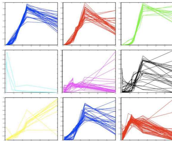
Figure 7: The nine clusters found by method EAC-DC(KL) with a modified coassoc criterion.
