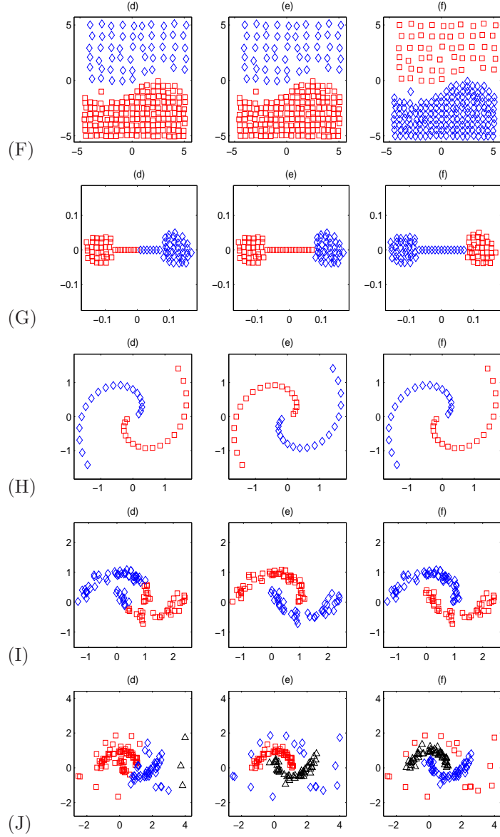
Figure 6: Data sets F to J are those already explored for Figure 3. Left(d) : Spectral clustering results on Euclidean distance; Middle(e): Spectral clustering of the complete heat kernelized DRPT affinity matrix; right(f) : same as (e), with DRPT affinity matrix estimated from M=N/4 partitions.
