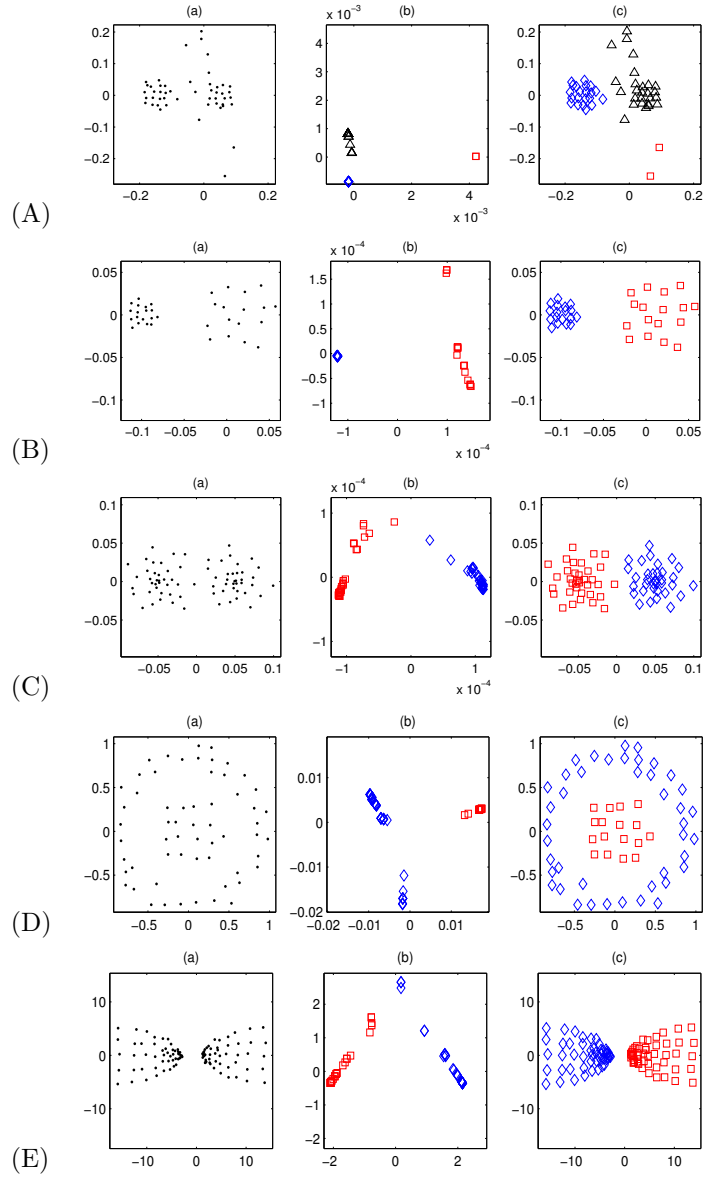
Figure 2: A: 2 identical clusters with outliers; B and E : 2 clusters with different densities; C: 2 identical clusters with variable densities; D: 1 annulus including a cluster. Left (a) : Data; Middle : DRPT-MDS embedded data; right : data labelled with clustering labels obtained by k-means method on the DRPT-MDS embedded data. Note that when outliers are present, k-means was set to search 3 clusters.
