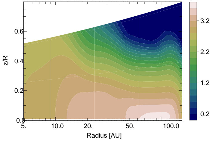
Fig. A.1. Map of the logarithm of the number of SPH particles per MCFOST grid cell in the meridional ( R, z/R ) plane for the 1 M_J planet.
