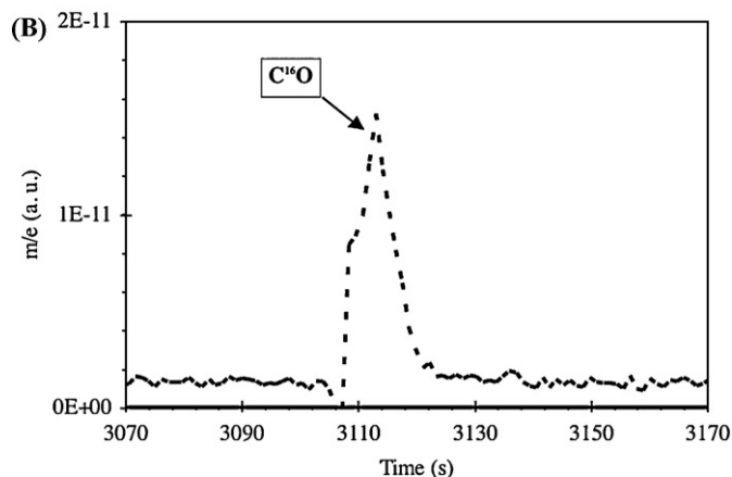
Fig. 9. Normalised oxygen-exchange transients over \text{AgMnO}_x at 300^\circ\text{C} . Conditions: 40 mg catalyst, total flow 50 mL/min, step 1: 20% ^{16}\text{O}_2 in argon, step 2: 20% ^{18}\text{O}_2 and 10% He in argon.
