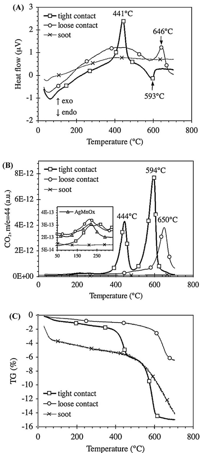
Fig. 5. DTA-TGA analysis of soot combustion under \text{N}_2 and different contact types (no catalyst, tight or loose contact with 3.5 wt.% \text{AgMnO}_x catalyst). (A) Heat flow profiles (data referred to 1 mg soot); (B) \text{CO}_2 analysed at the reactor outlet (data referred to 1 mg soot); (C) TG profiles. Conditions: 10 wt.% soot + 90 wt.% \text{AgMnO}_x catalyst in tight contact (35.08 mg sample) or loose contact (17.40 mg sample), or pure soot (3.82 mg sample), heating rate 5^{\circ}\text{C}/\text{min} , 50\text{ mL}/\text{min} \text{N}_2 .
