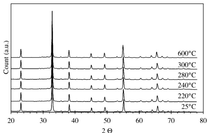
Fig. 6. In situ X-ray diffractograms of soot/3.5 wt.% \text{AgMnO}_x mixtures (10 wt.% soot) in tight contact vs. temperature, under \text{O}_2/\text{N}_2 . Conditions: 157 mg soot/catalyst mixture, 50% \text{O}_2/50\% \text{N}_2 , total gas flow rate 23\text{ mL}/\text{min} .
