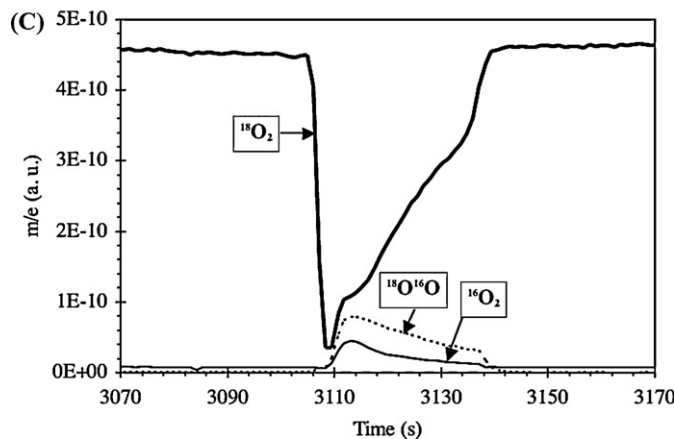
Fig. 10. Soot/ \text{AgMnO}_x combustion experiment under ^{18}\text{O}_2 . (A) \text{CO}_2 isotope profiles; (B) CO isotope profiles; (C) \text{O}_2 isotope profiles. Conditions: 10 wt.% soot + 90 wt.% \text{AgMnO}_x catalyst in tight contact (56.6 mg sample), 33% \text{O}_2 and 7% He in Ar (total flow rate 60 mL/min), heating rate 5^\circ\text{C}/\text{min} .
