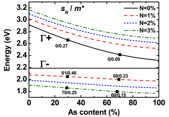
FIG. 2. (Color online) \Gamma- and \Gamma+ conduction bands for bulk Ga(NAsP) biaxially strained at different nitrogen concentrations at 0K. The energy reference is the same as in Fig. 1. The percentage of s_N contribution to the wave function is represented by the first number. The second number is the effective mass in the (100) direction in units of free electron mass m_0 .
