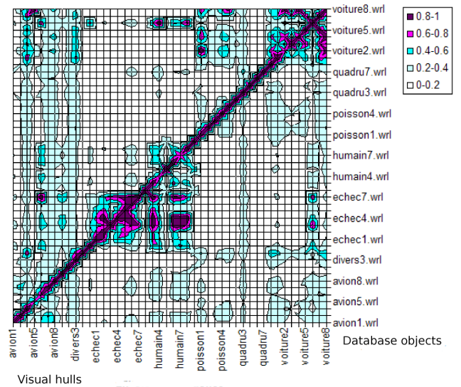
Figure 6. Gain matrix in spherical mode (12 views) with a field of view of 20° and 10% of outline points.
