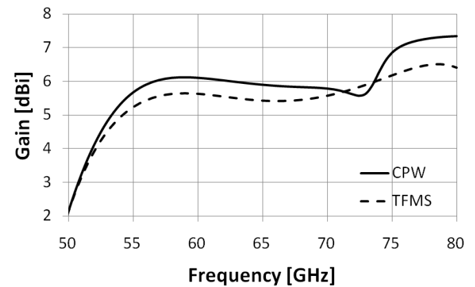
Fig.5 Simulated gain of the antenna with TFMS and CPW configurations.
