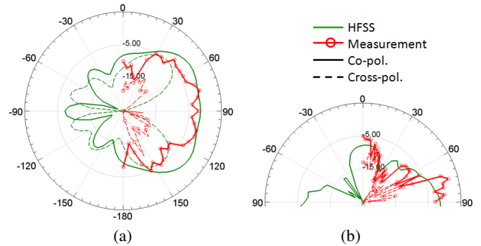
Fig.8 Measured and simulated radiation pattern of the antenna with CPW configuration on Alumina: E-plane (a) H-plane (b).
