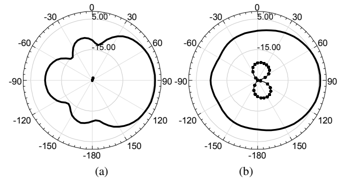
Fig.4 Radiation pattern of the CPW antenna configuration at 60 GHz: E Plane co/cross-Polarization (a) – H Plane co/cross-Polarization (b).
