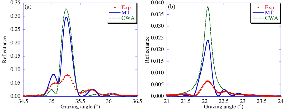
Figure 4: Comparison of the reflectivity curves obtained as a function of the angle and in the (a) B K and (b) C K ranges between the experiment (dots), simulation with the modal theory (solid line) and simulation with coupled-wave approach in the single-order regime (dotted line).
