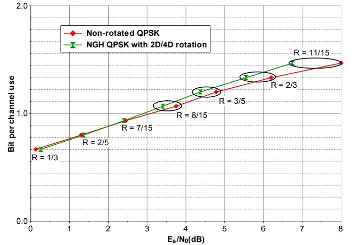
Figure 4. Performance gain due to the constellation rotation modes of DVB-NGH over memoryless Rayleigh channel. Both curves display the required SNR to achieve a FER= 10^{-4} after LDPC decoding.
